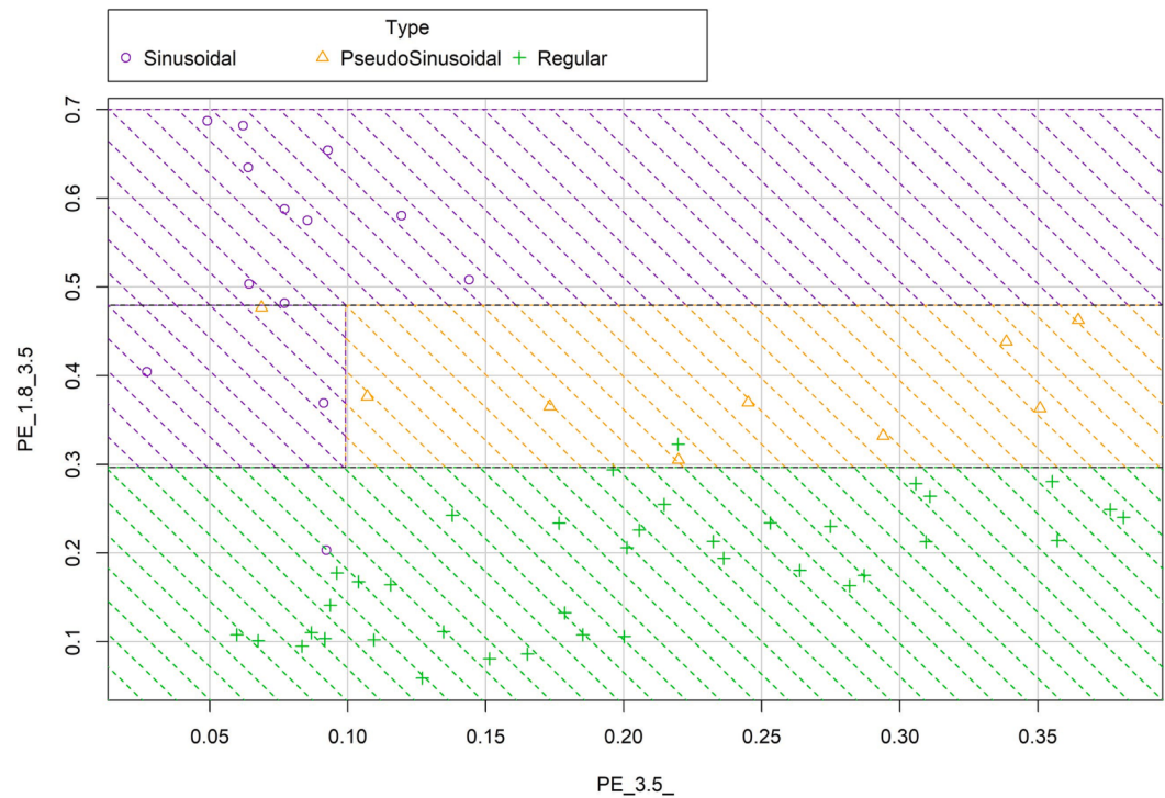
Fig. 3. Scatterplot of the 60 cases distributed by Proportion of energy in the interval frequency (1.8,3.5) and Proportion of energy_3.5_.
